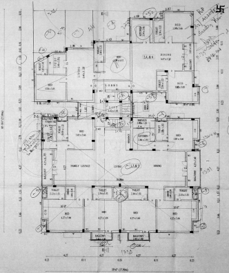
TYPICAL FLOOR PLAN (JUL & III FLOORS)
