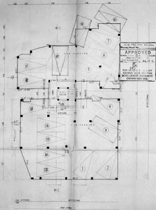
STILTS FLOOR PLAN
